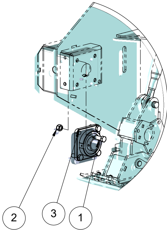
DETAIL A
